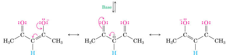
2,4-Pentandione ( pK_a = 9 )
