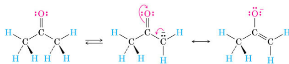
Acetone ( pK_a = 19.3 )
