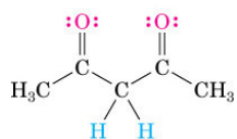
2,4-Pentandione ( pK_a = 9 )
