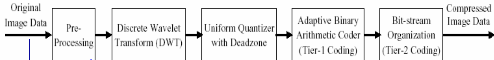
Fig. 1. JPEG 2000 fundamental building blocks.
