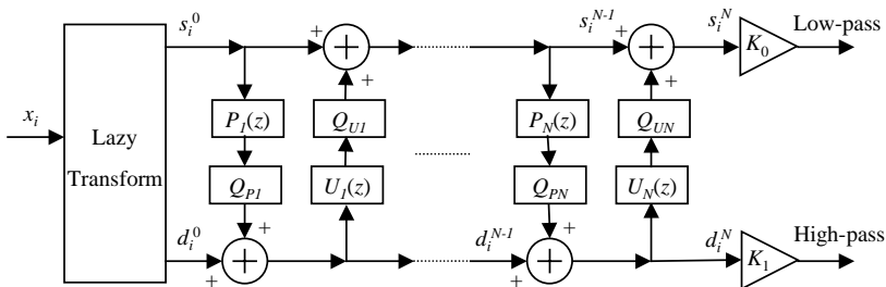
Fig. 9. General block diagram of a forward integer-to-integer transform using lifting.
